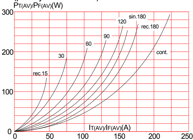
FIG.1: Power dissipation vs. on-state current (per thyristor or diode)
