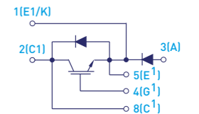
Chopper Low Side - PLM
