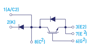
Chopper Low Side - PLM
