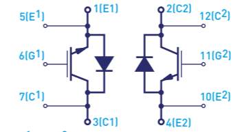
Dual Switch - DDM/S
