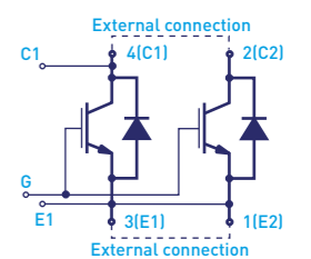
Single Switch - NSM
