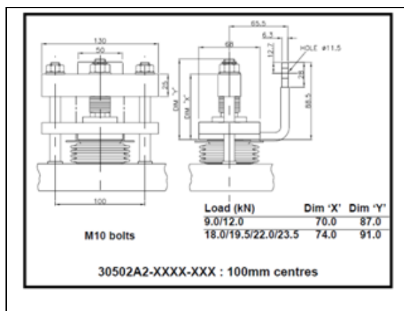
Figure 6 Typical Clamp for Single Side Cooling
